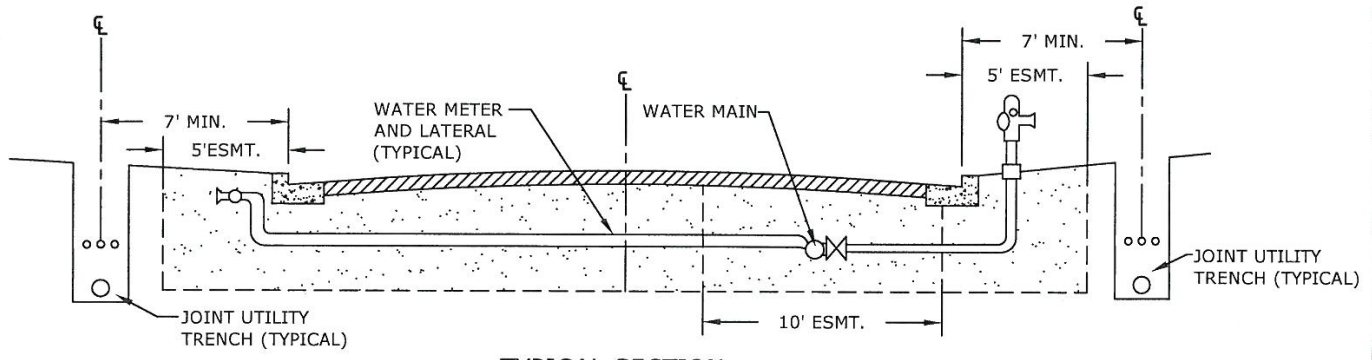
TYPICAL SECTION
